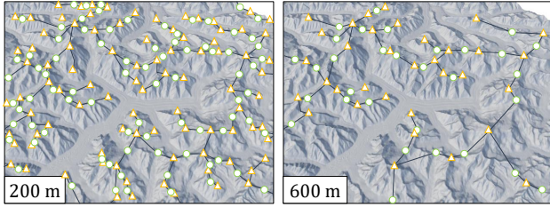
Figure 38: Identified peaks and key saddles with two prominence thresholds. Orange: peaks, green: saddles. Black edges represent the connectivity of the Divide tree (Section 7.3).
