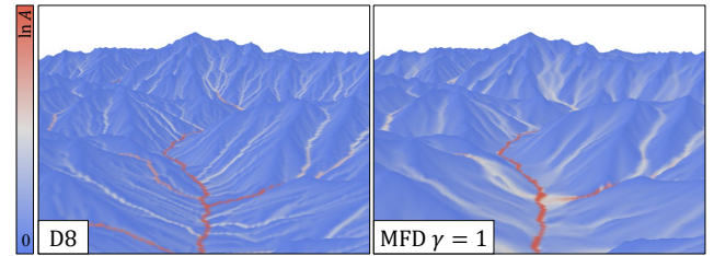
Figure 30: Single-direction (D8) and multiple direction (MFD) computation of drainage area A .
