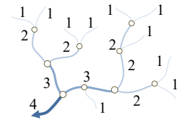
Figure 44: Horton-Strahler ordering.
