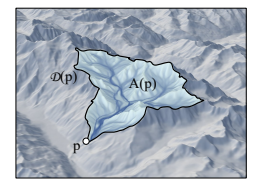
Figure 32: Drainage basin and drainage area.
