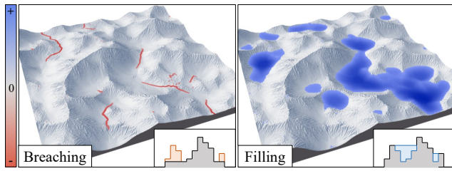
Figure 31: Depression breaching and depression filling on a noise turbulence terrain.
