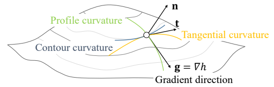
Figure 6: Illustration of different types of curvatures.
